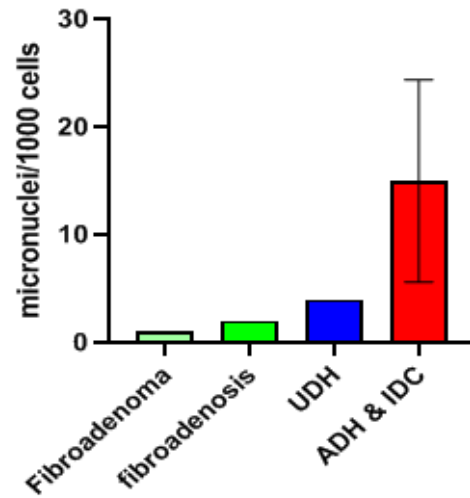
Fig. 2: Micronuclei among various groups
